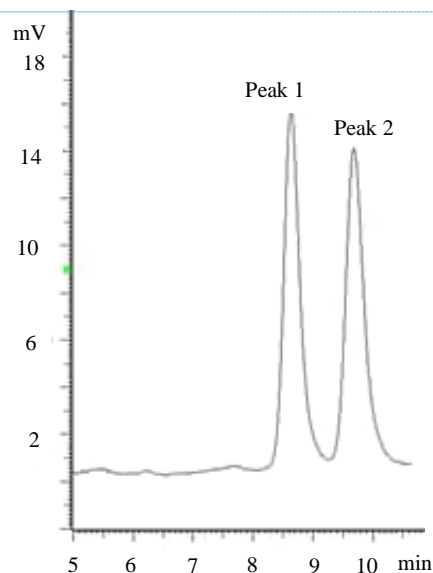
Figure 2. Chromatogram of econazole enantiomers in the pharmaceutical (liquid) sample.
