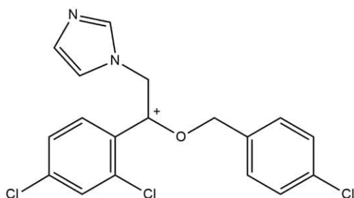
Figure 1. Chemical structure of econazole
